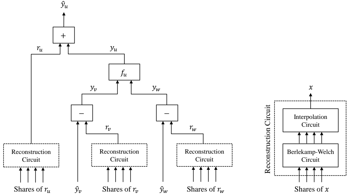
Figure 2.3: Circuit of gate u
